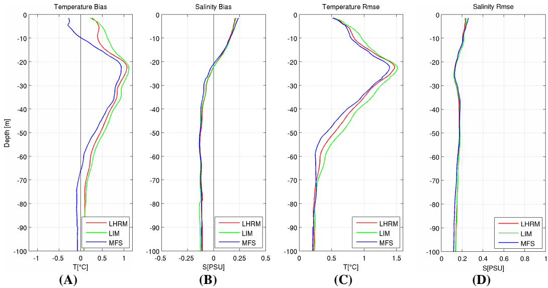
Figure 4.16 Averaged vertical profiles for the upper 100m for: (A) temperature bias, (B) salinity bias, (C) temperature RMS error, (D) salinity RMS error. Blue lines indicate MFS results, green lines LIM results and red lines LHRM results for Exp2A.
