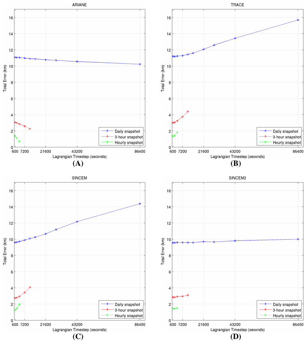
Figure 2.11 CASE3. Total error values (km) for Experiments 2-19 against Lagrangian timestep (seconds), for: ARIANE (A), TRACE (B), SINCEM (C) and SINCEM2 (D) algorithms. The different coloured lines refer to experiments with different temporal frequency currents snapshots.
