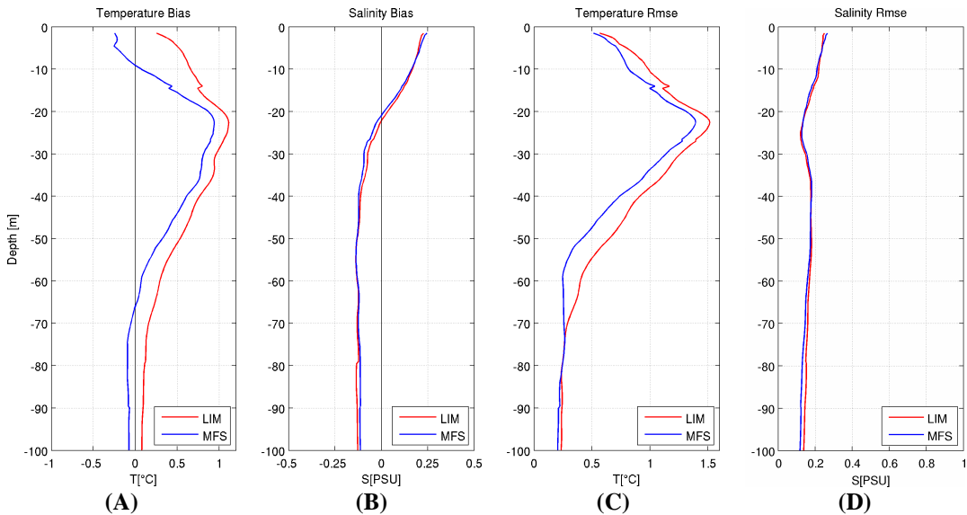
Figure 4.11 Averaged vertical profiles for the upper 100m for: (A) temperature bias, (B) salinity bias, (C) temperature RMS error, (D) salinity RMS error. Blue lines indicate MFS results and red lines LIM results for Exp2.
