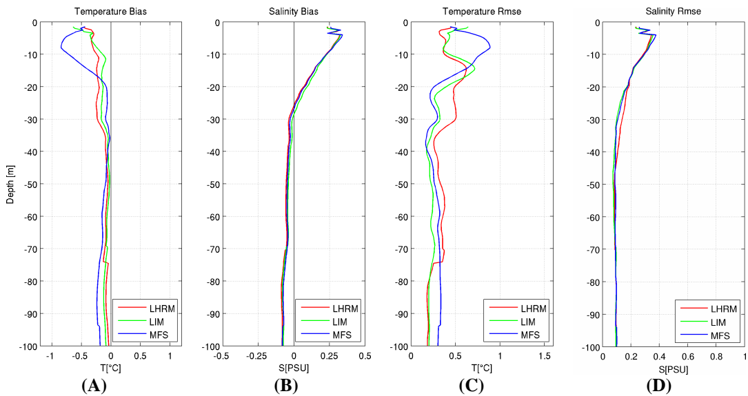
Figure 4.15 Averaged vertical profiles for the upper 100m for: (A) temperature bias, (B) salinity bias, (C) temperature RMS error, (D) salinity RMS error. Blue lines indicate MFS results, green lines LIM results and red lines LHRM results for Exp1A.
