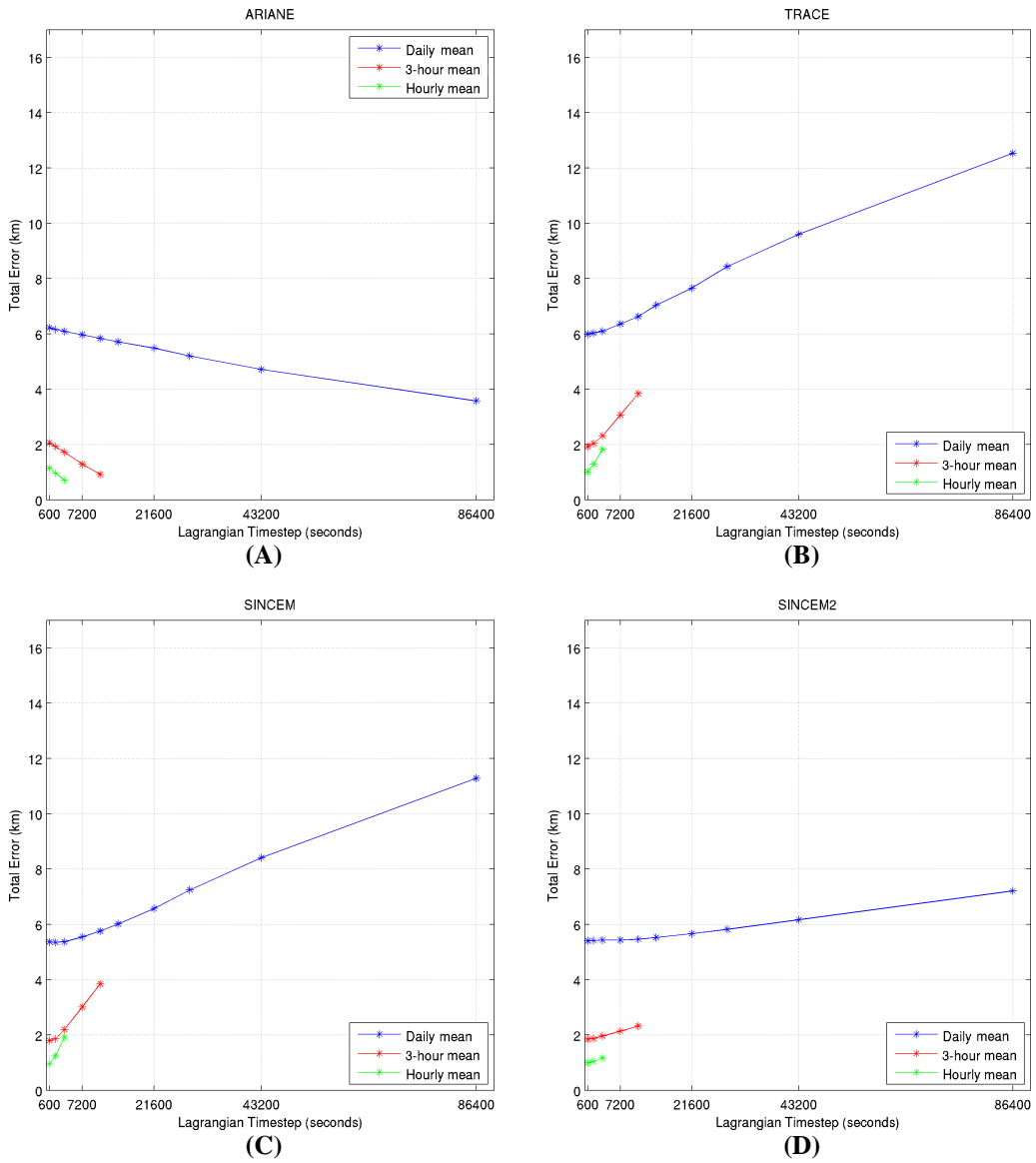
Figure 2.9 CASE1. Total error values (km) for Experiments 2-19 against Lagrangian timestep (seconds), for: ARIANE (A), TRACE (B), SINCEM (C) and SINCEM2 (D) algorithms. The different coloured lines refer to experiments with diverse temporal frequency currents.
