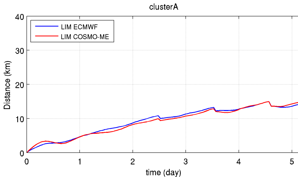
Figure 5.8 Ensemble average of the distance errors between drifters and simulated particles in function of the simulation time for clusterA.
