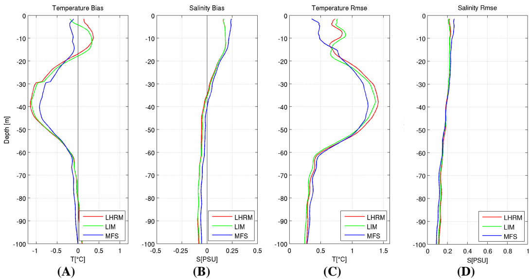
Figure 4.17 Averaged vertical profiles for the upper 100m for: (A) temperature bias, (B) salinity bias, (C) temperature RMS error, (D) salinity RMS error. Blue lines indicate MFS results, green lines LIM results and red lines LHRM results for Exp3A.
