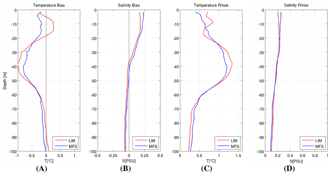
Figure 4.12 Averaged vertical profiles for the upper 100m for: (A) temperature bias, (B) salinity bias, (C) temperature RMS error, (D) salinity RMS error. Blue lines indicate MFS results and red lines LIM results for Exp3.
